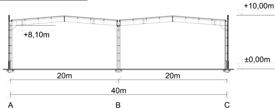
CROSS SECTION
