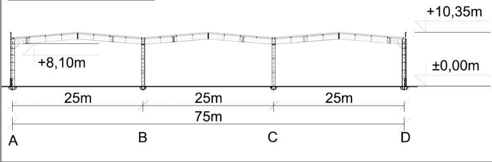
CROSS SECTION
