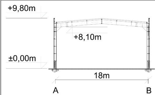
CROSS SECTION 6.2.1
