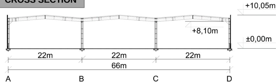
CROSS SECTION
