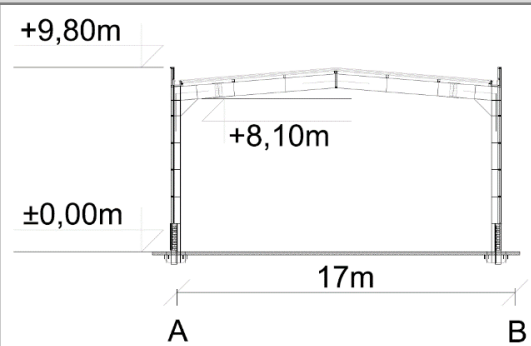
CROSS SECTION 6.2.2
